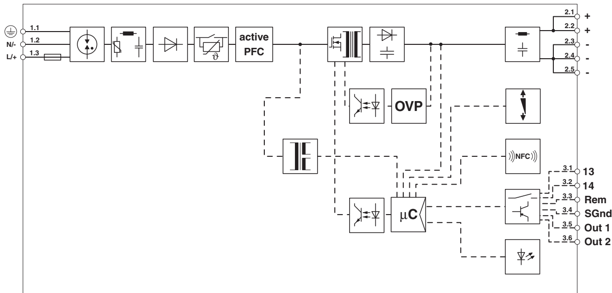
Block diagram
